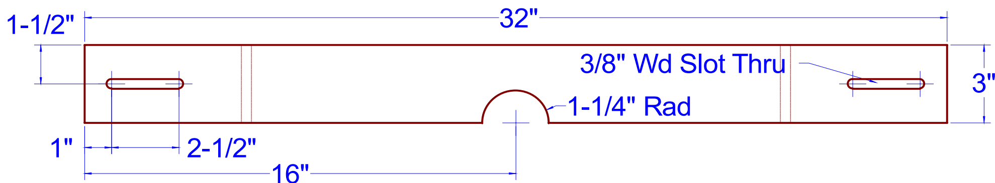
Face View
