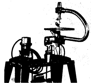
COMPRESSOR / SPRAYER-JIG SAW — popular set-up shown includes pulley guard, mounting bases and double-shaft motor.
