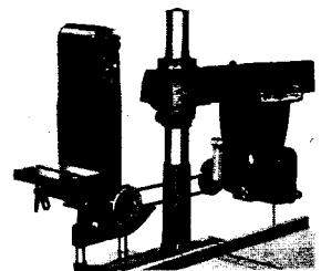
For mounting on Sawsmith, use 505635 (27920) Bracket and 505636 (27924) Belt and Pulley Kit
