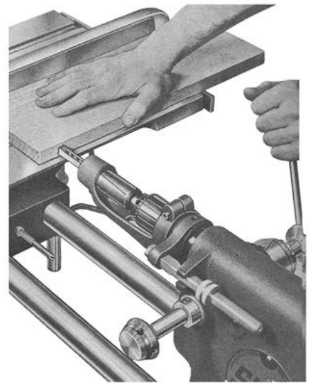
MORTISING, in Horizontal Position
