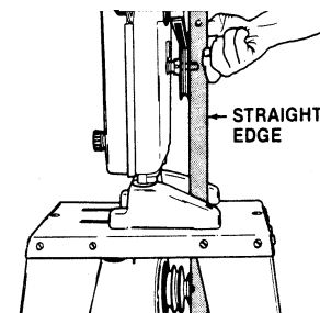
Figure 1 - Use a straightedge to align the pulleys.
