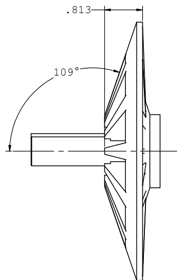
504180 IDLER SHEAVE
