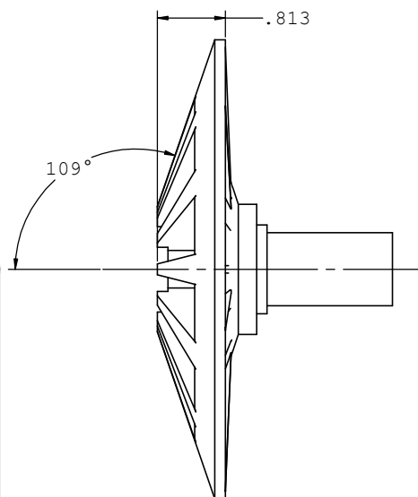
504181 CONTROL SHEAVE
