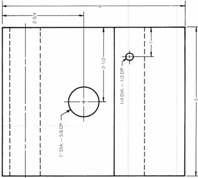
HEADSTOCK "J" 4-1/4" x 5" x 6"
