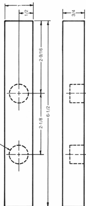
EXTENSION TABLE "V" 3/4" x 1" x 6-1/2"
